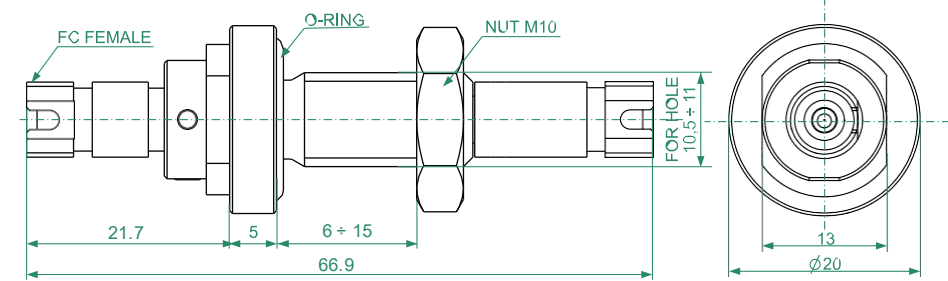
Fiber Optic Feedthrough Type M10
